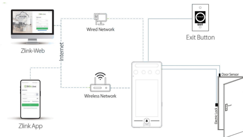
BEST Protocol
