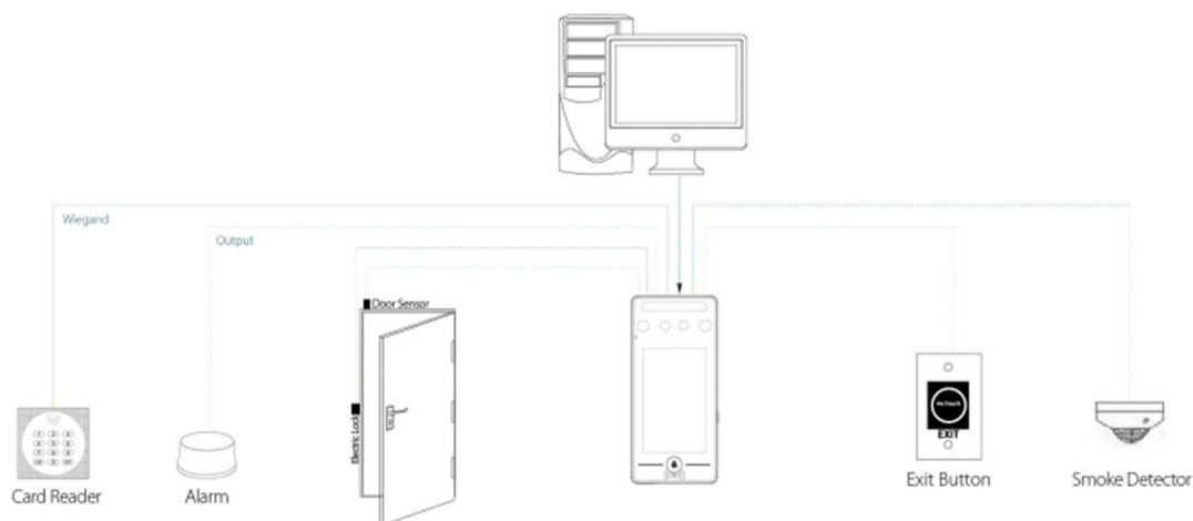
PUSH Protocol
